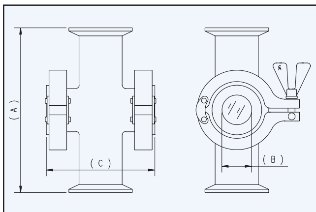
DIMENSIONS (mm/inches)
