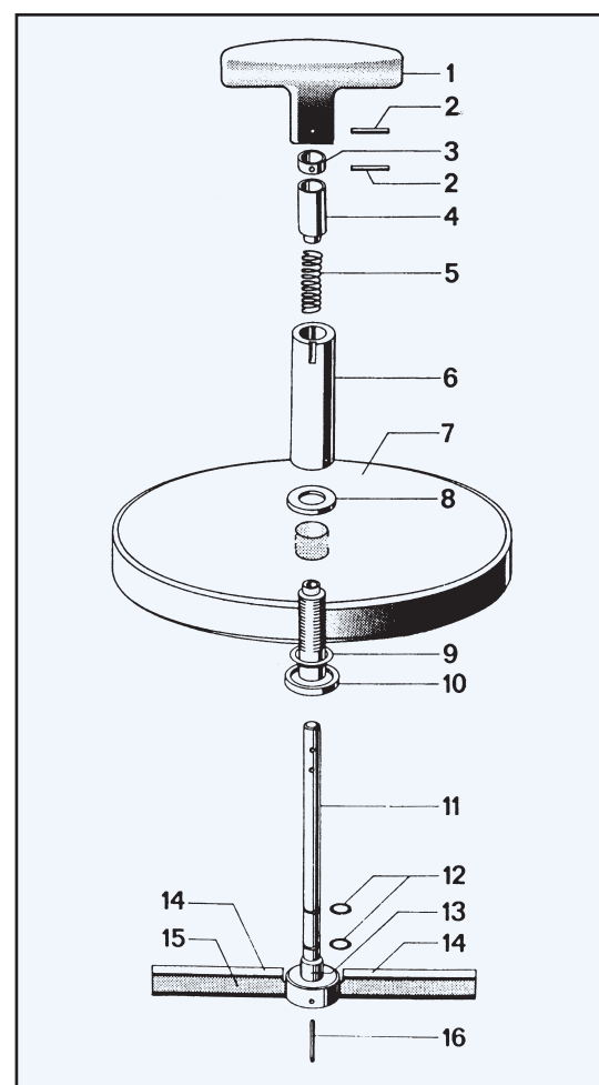
Exploded view of components
